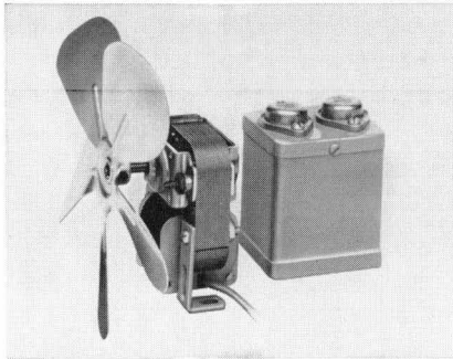
Fig. 1. New PAECO fan enables long life and quietness of ac fan motor to be obtained in variable line frequency applications.
