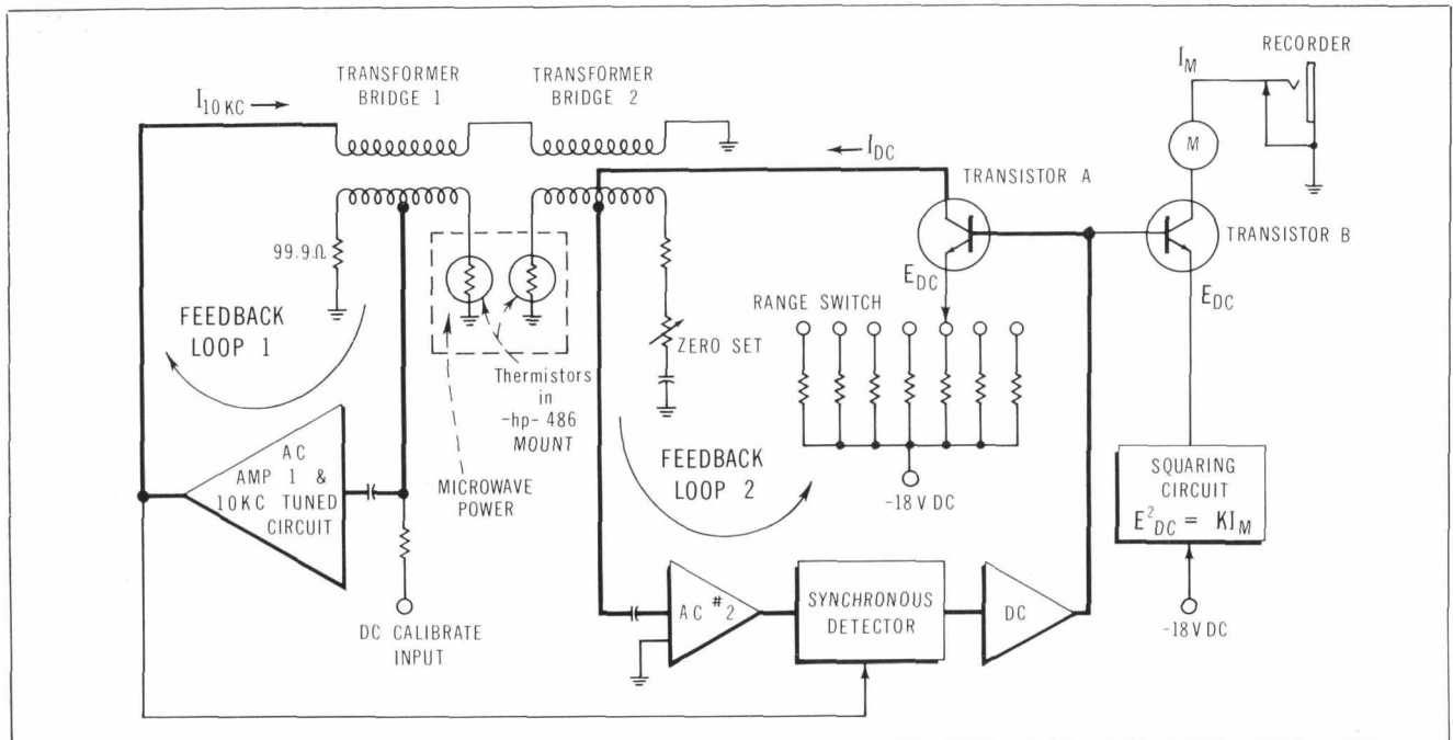
Fig. 3. Basic circuit arrangement of -hp-431A Power Meter. High thermal stability occurs from use of double-bridge technique with compensated thermistor mounts.
