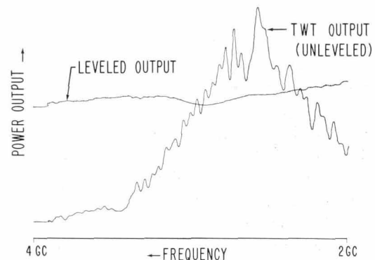
Fig. 2. Comparison of unlevelled output of traveling-wave tube amplifier with output when leveled using new power meter in arrangement described in text.
